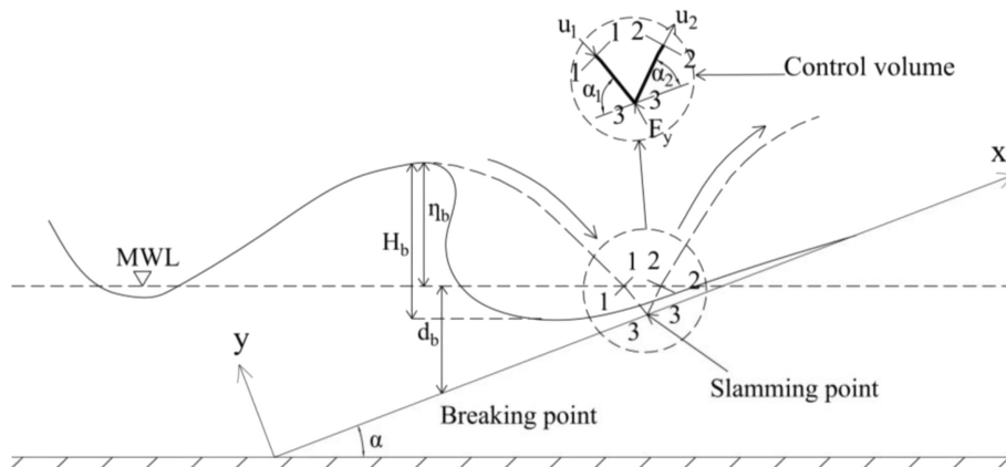
Fig. 1. Wave breaking on a dike slope – principle sketch and control volume.
