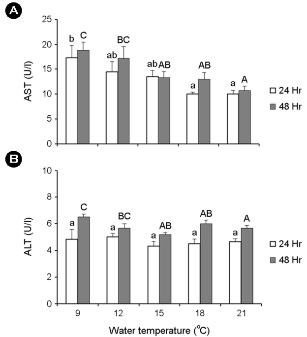
Fig. 4. Plasma AST (A) and ALT (B) of olive flounder, Paralichthys olivaceus in different water temperature at the conclusion of this experiment. Data were expressed as mean ± S.E. (n=10). Different letters denote significant difference among each group (p < 0.05).
