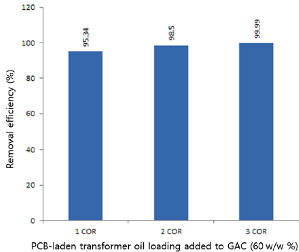
Figure 6. Removal efficiency after 1, 2, 3 COP with insulating oil loading added to GAC (60 w/w %).
