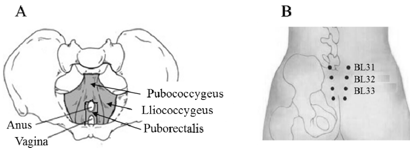
Fig. 2. Levator ani muscles (A) and Acupoints (BL31 to BL33)
