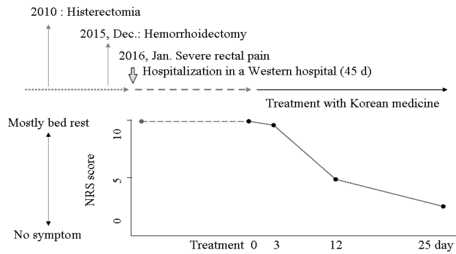
Fig. 3. Summary of clinical courses and treatment outcome
