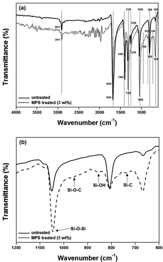
Figure 2. FTIR spectra of untreated and MPS treated polyketone fiber (a) 4000~600 \text{cm}^{-1} , (b) 1200~600 \text{cm}^{-1} .
