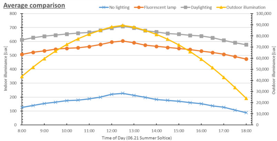
Fig. 11 Change of average indoor illuminance with time
