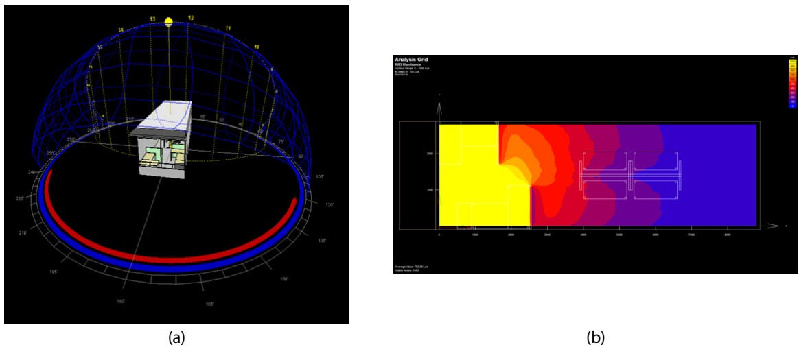
Fig. 4 Solar altitude and indoor illuminance (simulated) (a) summer solstice (b) result: at 12:30 blind 50%
