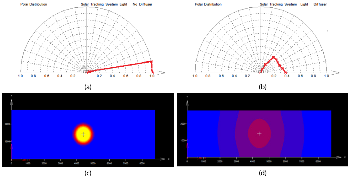
Fig. 9 Diffuser setting; (a) No diffuser (b) Diffuser (c) Before applying the diffuser (d) After applying the diffuser
