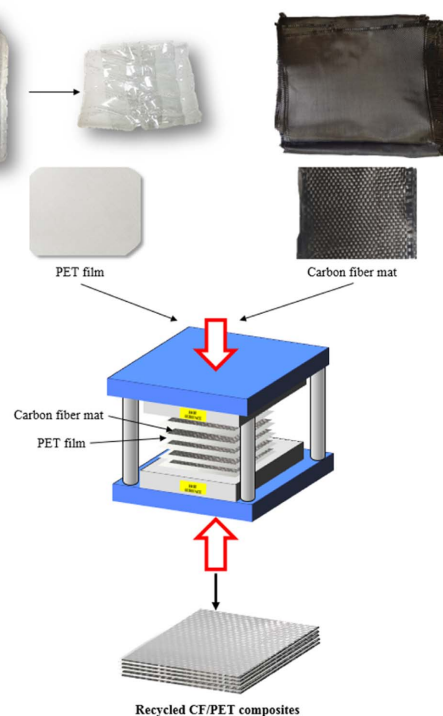
Fig. 1. Schematic arrangement of manufacturing process for recycled PET composites
