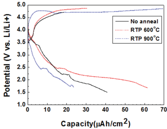
Fig. 8. Charge-discharge curves of the \text{Li}_2\text{MnSiO}_4 cathode thin films with and without annealing by RTP. The RTP temperature was 600°C or 900°C. Only liquid electrolyte was adopted.
