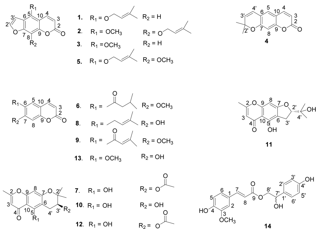
Fig. 1. Structures of 1 – 14.
