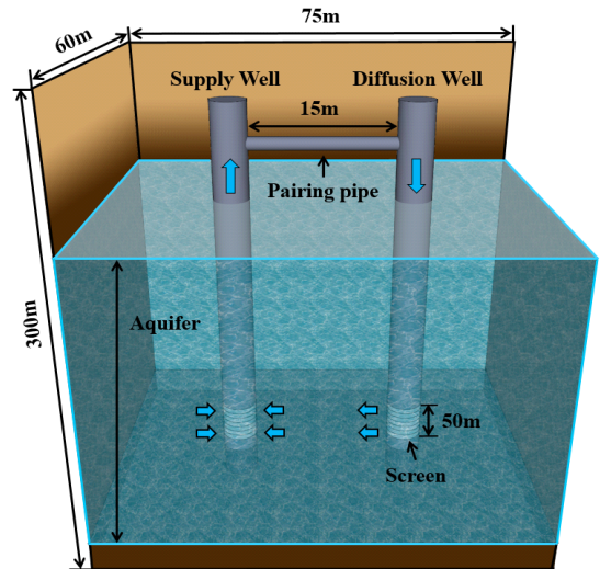
Fig. 2. Simulation model
