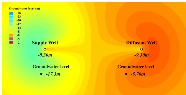
Fig. 5. Groundwater level of wells (Case 1-3, k:1 \times 10^{-7} \text{ m/s} , 2/28)
