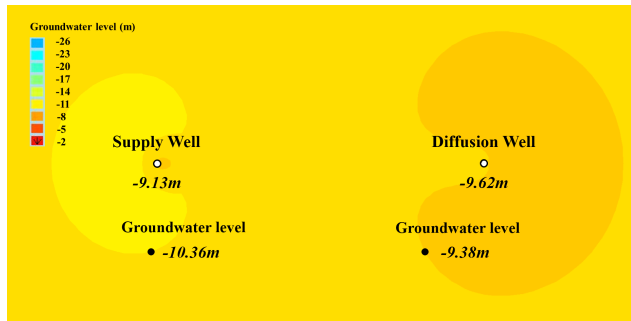
Fig. 3. Groundwater level of wells (Case 1-1, k:1 \times 10^{-6} \text{ m/s} , 2/28)
