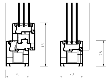
Fig. 5 Tilt & turn triple glazed window
