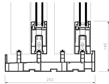
Fig. 4 4(Four)-Track sliding window
