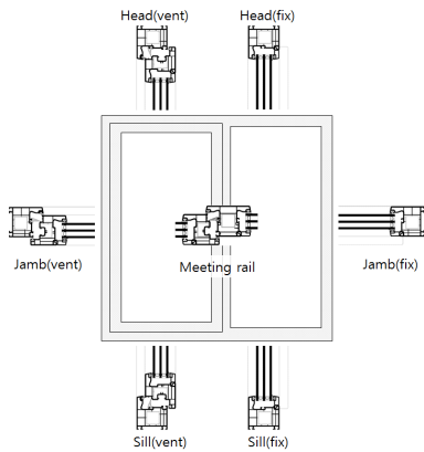
Fig. 7. Composition of tilt & turn triple glazed window
