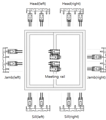
Fig. 6 Composition of 4-track sliding window
