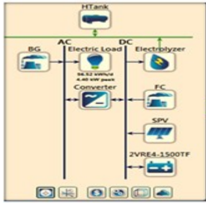
Fig. 8. The proposed system architecture of this HRES
