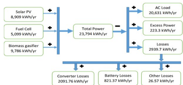
Fig.14. Energy flow diagram of proposed HRES
