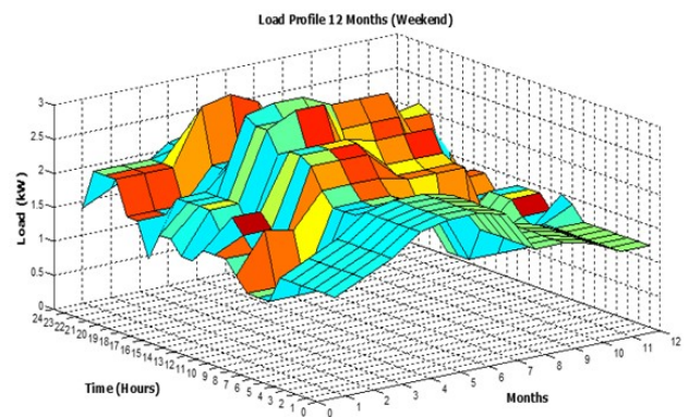
Fig. 5. 3D surface plot of 12-month load profile weekend day
