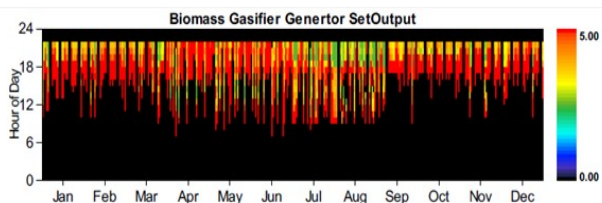
Fig. 10. Monthly average power of 5 kW downdraft biomass gasifier
