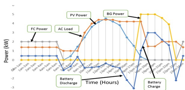
Fig. 15. Power flow diagram of proposed HRES
