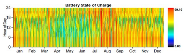
Fig. 13. Battery state of charge (SOC) in different month of a year
