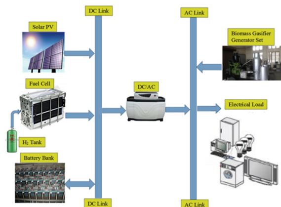
Fig. 1. Block diagram of proposed HRES
