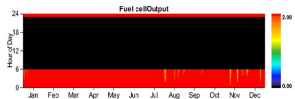
Fig.12. Monthly average power of 2 kW fuel cell
