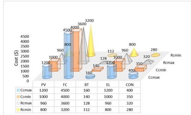
Fig. 6. Cost analysis of different components of proposed HRES
