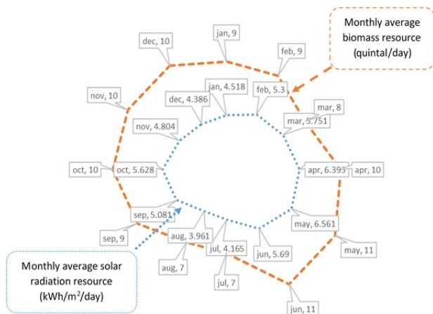
Fig. 3. Monthly average solar radiation and biomass resources
