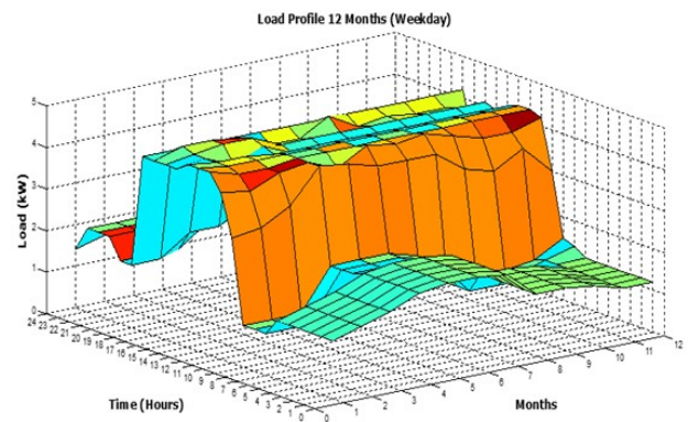
Fig. 4. 3D surface plot of 12-month load profile weekday days
