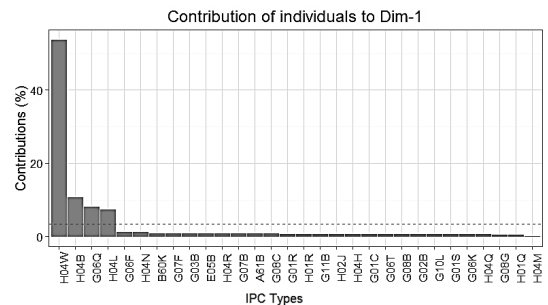
Fig. 3. Contribution of variables to PC1(Mean = 3.2222)
