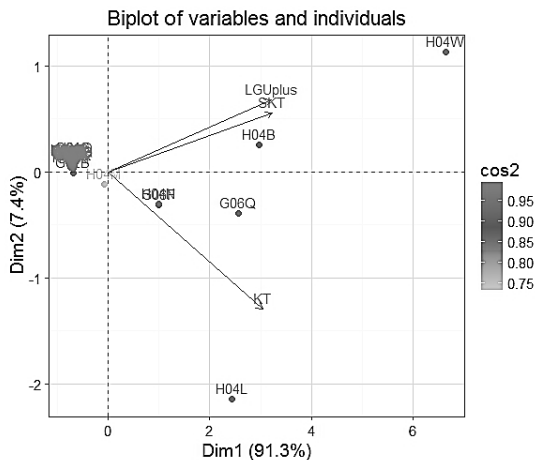
Fig. 4. Variables and Individuals Biplot (PC : 1~2)
