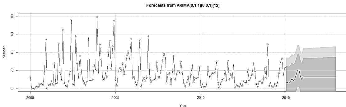
Fig. 8. ARIMA Model Forecast Result<ARIMA(0,1,1)(0,0,1)[12], Confidence Interval : 80%/95%> of H04L
