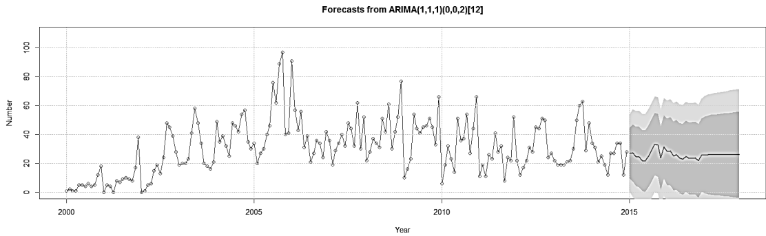
Fig. 5. ARIMA Model Forecast Result<ARIMA(1,1,1)(0,0,2)[12], Confidence Interval : 80%/95%> of H04W
