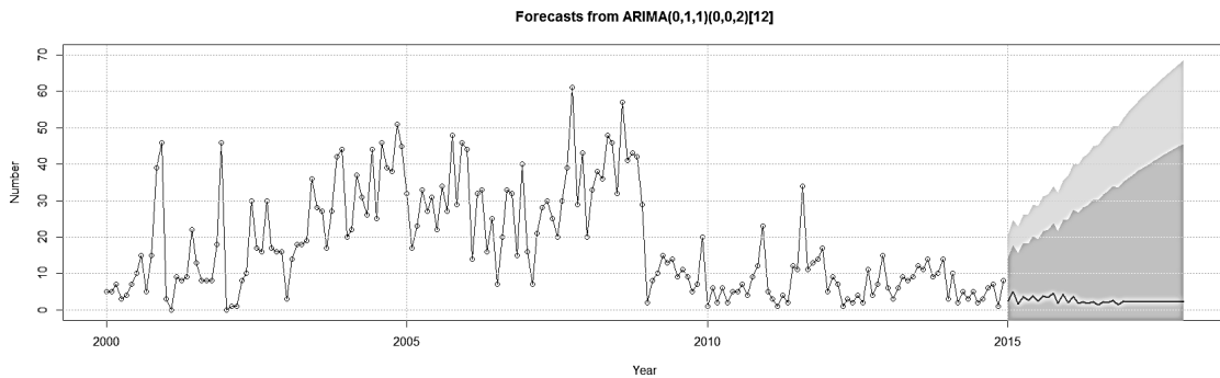
Fig. 6. ARIMA Model Forecast Result<ARIMA(0,1,1)(0,0,2)[12], Confidence Interval : 80%/95%> of H04B
