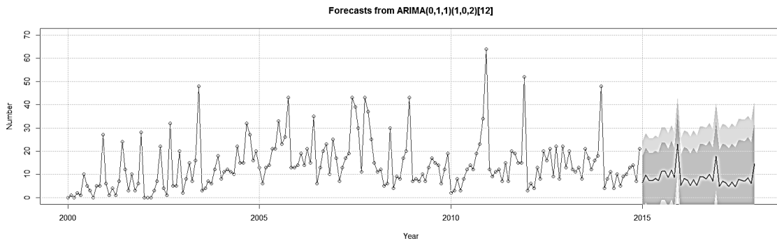
Fig. 7. ARIMA Model Forecast Result<ARIMA(0,1,1)(1,0,2)[12], Confidence Interval : 80%/95%> of G06Q
