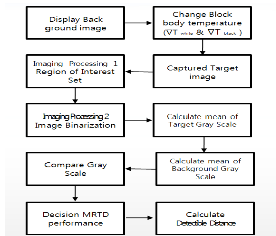
Fig. 7. MRTD performance decision algorithm
