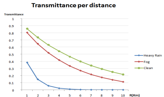
Fig. 10. Transmittance per distance
