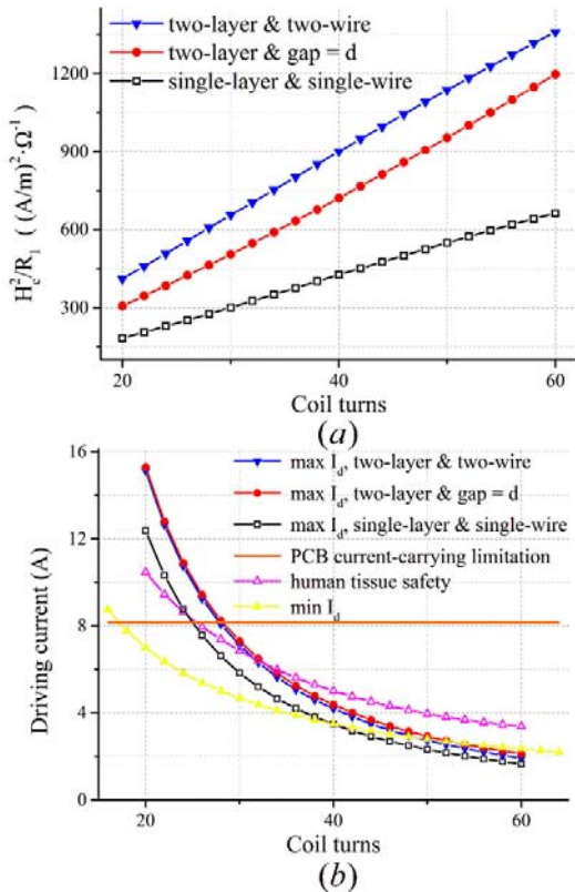
Fig. 13. The calculated H_c^2/R_1 and the permissible I_d varying with n_t at 220 KHz for transmitting coils with the type A, D and F topologies in Table I.
