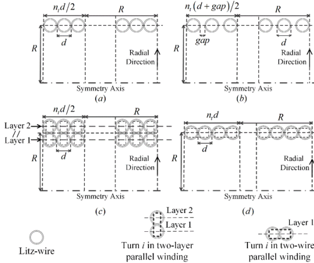
Fig. 3. Topologies of transmitting coils. (a) Single-layer tightly wound coil. (b) Coil with spaced winding. (c) Coil with parallel layer winding. (d) Coil with parallel wire winding.
