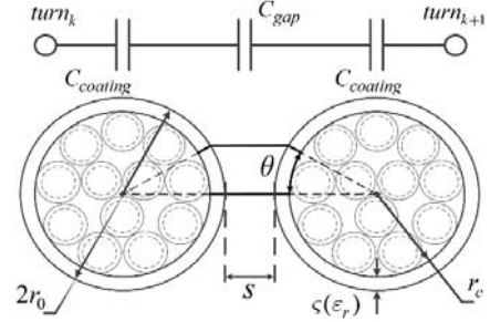
Fig. 6. Equivalent model of the turn-to-turn stray capacitance.
