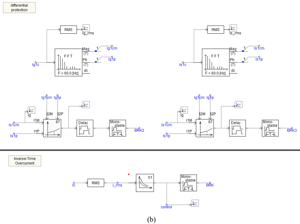
Fig.13. Simulation model in PSCAD. (a) Microgrid model. (b) Protection model.
