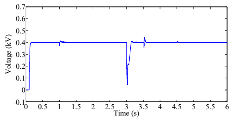
Fig. 20. Voltage of a Microgrid in the islanded mode.
