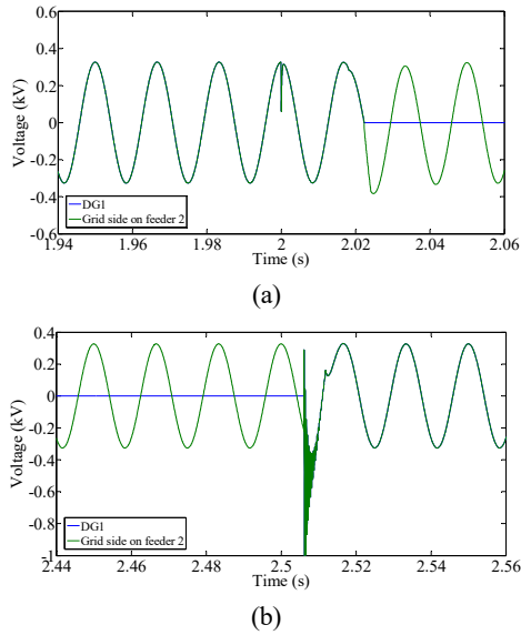
Fig. 17. Simulated voltage of phase C in feeder 2 under a three phase fault (fault 2). (a) Voltage variation during fault 2. (b) Voltage variation after isolating fault 2.
