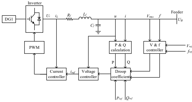
Fig. 3. V - f control.
