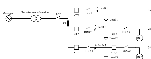
Fig.1. A typical Microgrid system.
