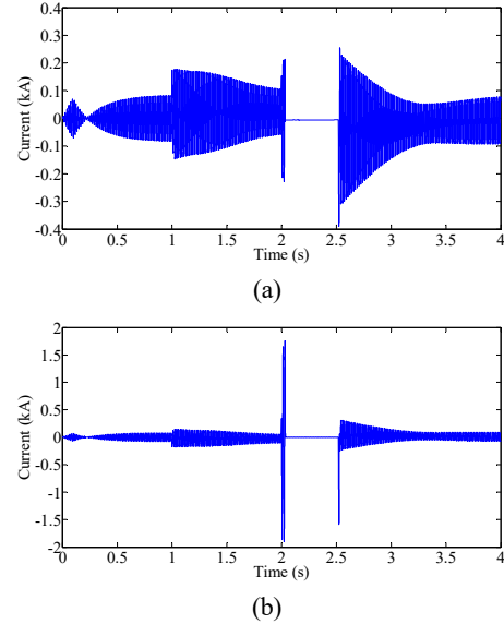
Fig. 19. Phase C current in feeder 3 under a phase C to ground fault (fault 3). (a) Current in the grid side. (b) Current in the DG2 side.
