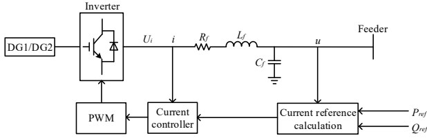
Fig. 2. P - Q control.
