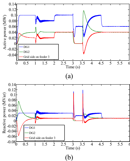
Fig.22. Active power and reactive power in both the DG2 side and the grid side under a three phase fault (fault 3). (a) The active power. (b) The reactive power.
