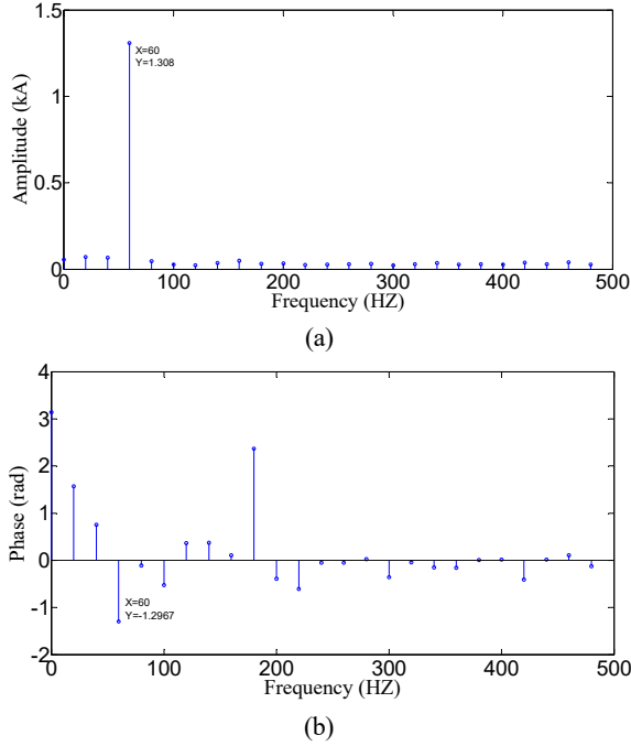
Fig. 11. Amplitude and phase values of the DG1 side fault current in the frequency domain under fault 2. (a) The amplitude value. (b) The phase value.
