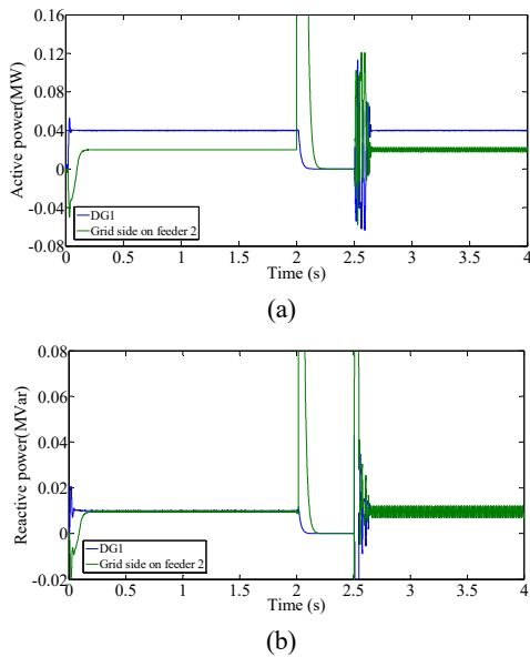
Fig. 18. Simulated active power and reactive power in the DG1 side and grid side under a three phase fault (fault 2). (a) Active power. (b) Reactive power.
