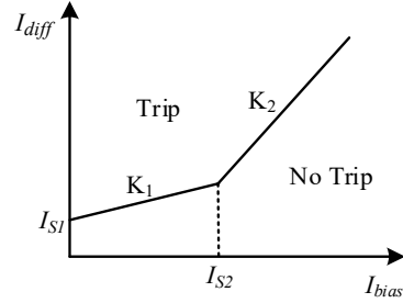
Fig. 10. Characteristic of the biased differential protection.
