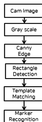
Fig. 7. Marker Detection Flowchart
