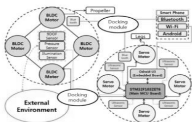
Fig. 4. Technical Architecture
