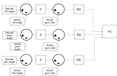
Fig. 6. P-PID Controller
