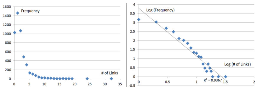
Figure 2 Distribution of the number of nodes in computer research network
