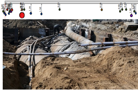
Fig. 1. Example photograph, Life-Lines of underground on the road
