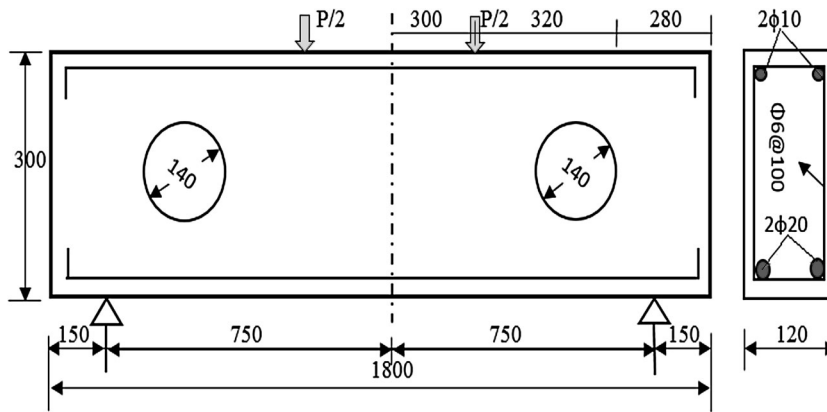
Fig. 1 Specimen's details (in mm).
