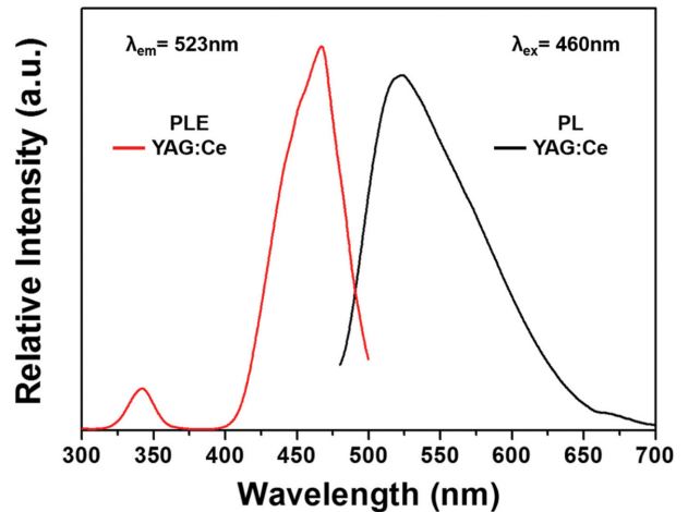
Fig. 3. Photoluminescence of synthesized YAG : Ce 3+ .
