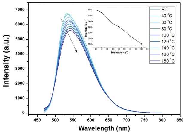
Fig. 4. Thermal quenching of synthesized YAG : Ce 3+ and comparison among the maximum value of intensity in each temperature.
