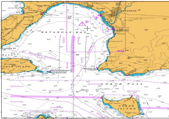
[Fig. 5] Batangas Bay & Verde Is Passage TSS
