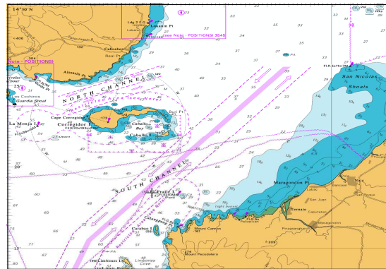
[Fig. 4] Entrance to Manila Bay - Northern and Southern Channels - TSS
