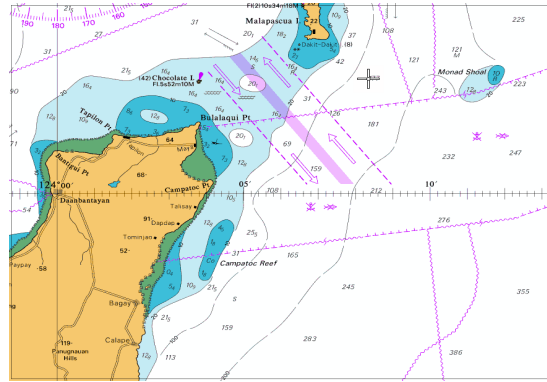
[Fig. 7] Chocolate Is. (Camotes Sea) TSS
