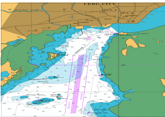
[Fig. 6] Southern entrance TSS to Cebu
