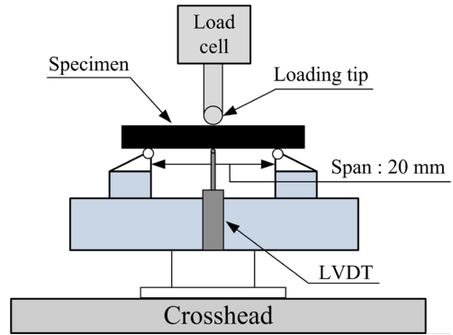
Fig. 3. Overview of interlaminar shear strength test
