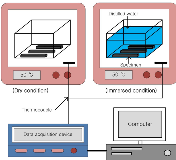
Fig. 2. Configuration of environmental test equipments
