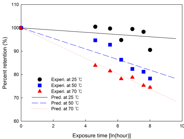
Fig. 7. Interlaminar shear strength and linear regression lines for the specimens exposed to immersion condition at 25°C, 50°C, and 70°C
