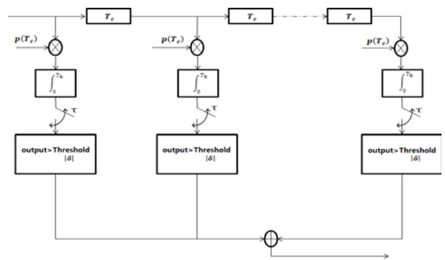
Figure 8: RAKE processing with threshold
