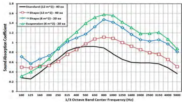
Figure 7: comparing sound absorption coefficients depending on each working method
