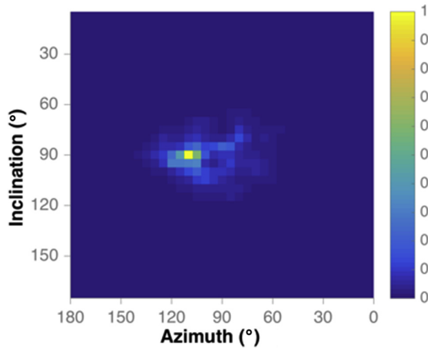
Fig. 3. Neutron image reconstructed using SOE. SOE, stochastic origin ensemble.
