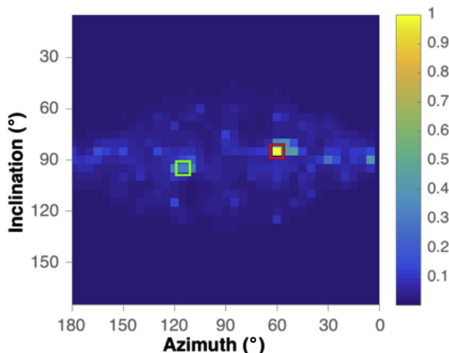
Fig. 4. Photon image reconstructed using SOE. SOE, stochastic origin ensemble.
