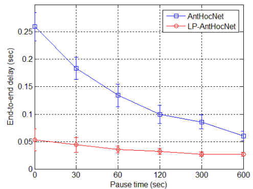
Fig. 8. Comparison of end-to-end delay.
