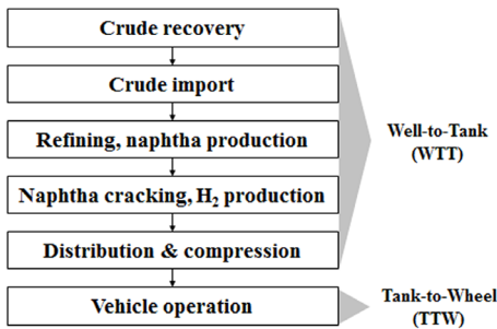
Fig. 2 WTT process of FCEV
