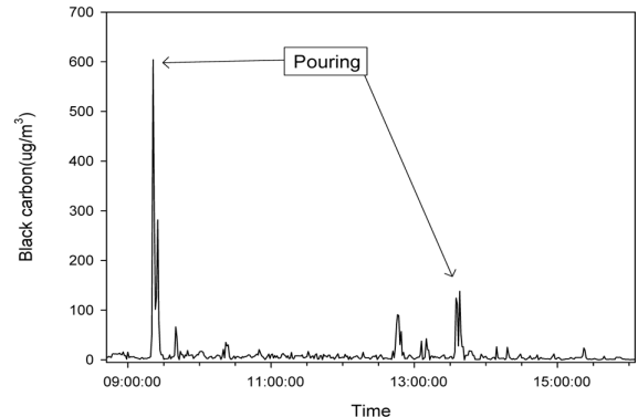
Figure 3. Real-time airborne black carbon concentration in furnace worker
