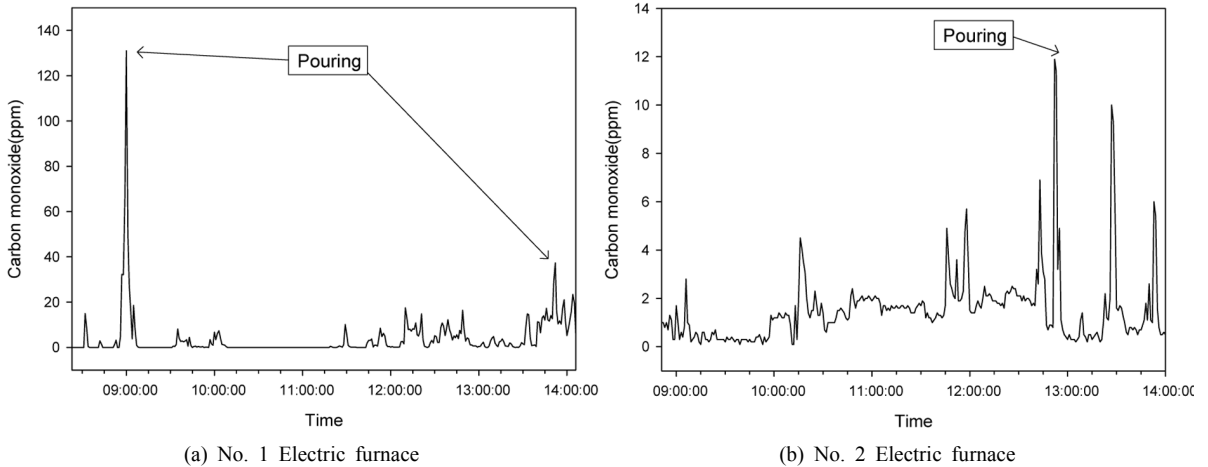
Figure 2. Real-time airborne carbon monoxide concentration in furnace worker
