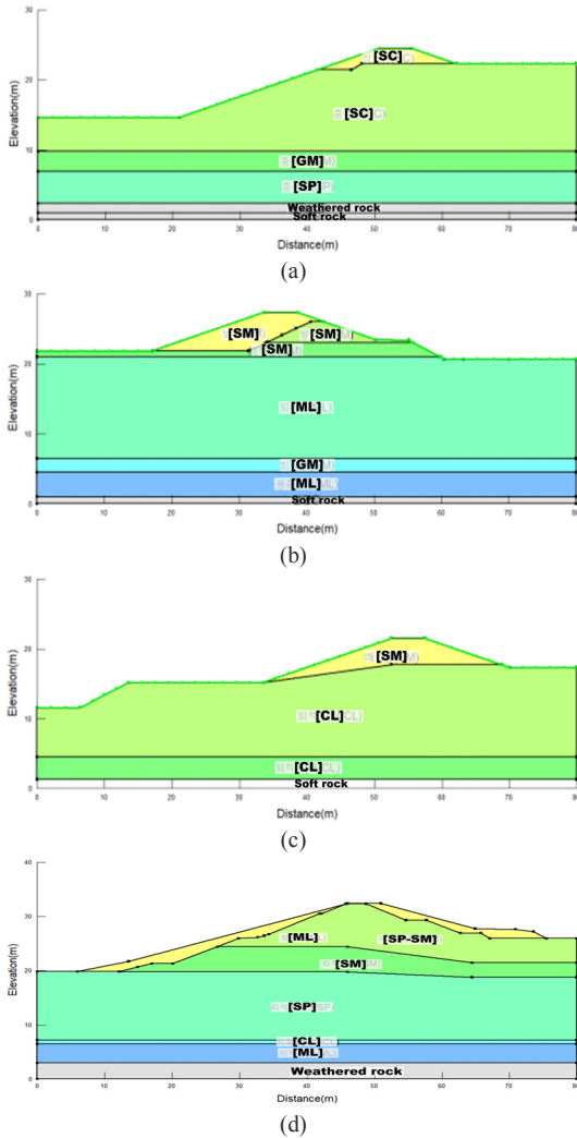
Fig. 5. Levee cross-section used in numerical analysis (a)R1 (b)R2 (c)R3 (d)R4
