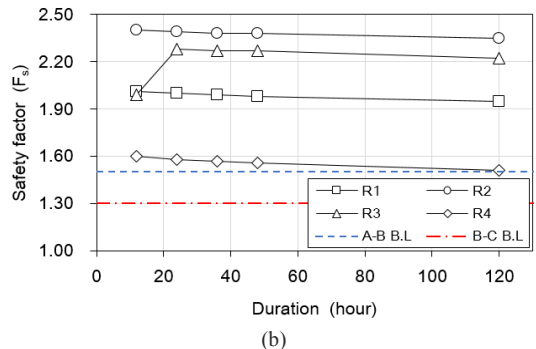
Fig. 6. Result of numerical analysis - Sliding (a) Landside (b) Riverside
