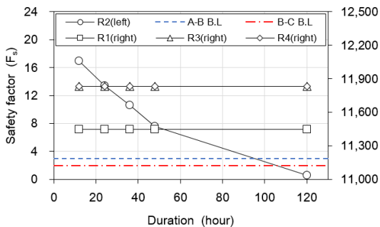
Fig. 7. Result of numerical analysis - Piping
