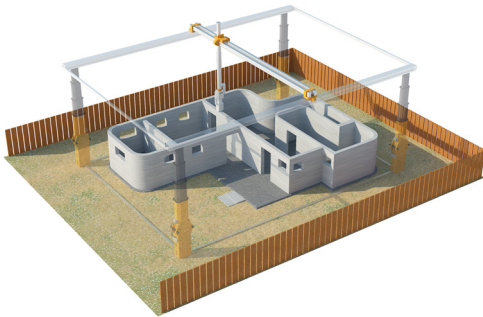
Fig. 9. Test model and 3D printer image
