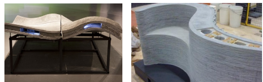
Fig. 4. Freeform Construction (IMCRC Center)
