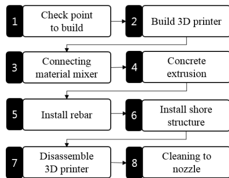
Fig. 8. 3D printing process for construction
