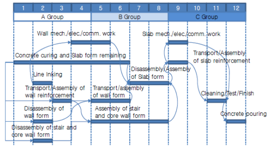
Fig. 7. 12 days typical floor structural work schedule[6]
