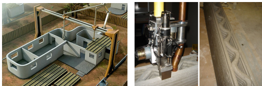
Fig. 3. Contour Crafting (USC)
