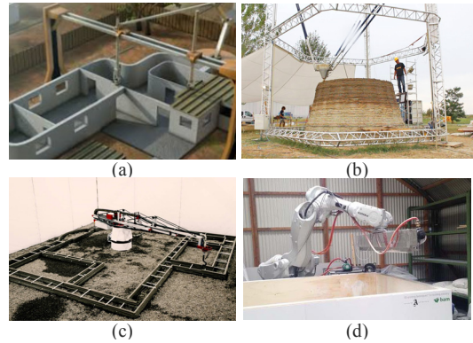
Fig. 6. Types of 3D printing (a)Gantry Type (b)Delta Type (c)Crane Type (d)Multi-joint Robot Type
