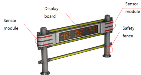
Fig. 6. Crosswalk smart fence
