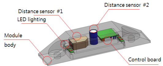
Fig. 10. Configuration of sensor module
