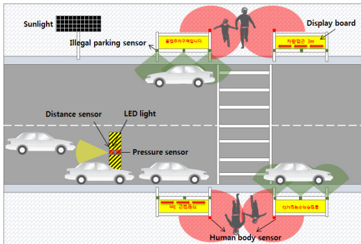
Fig. 4. Traffic safety facilities design concept
