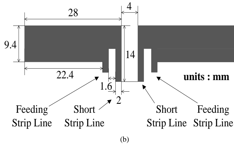
Fig.2. Geometry of the proposed antenna. (a) Proposed PIFA vs Coupling antenna, (b) PIFA vs PIFA antenna.
