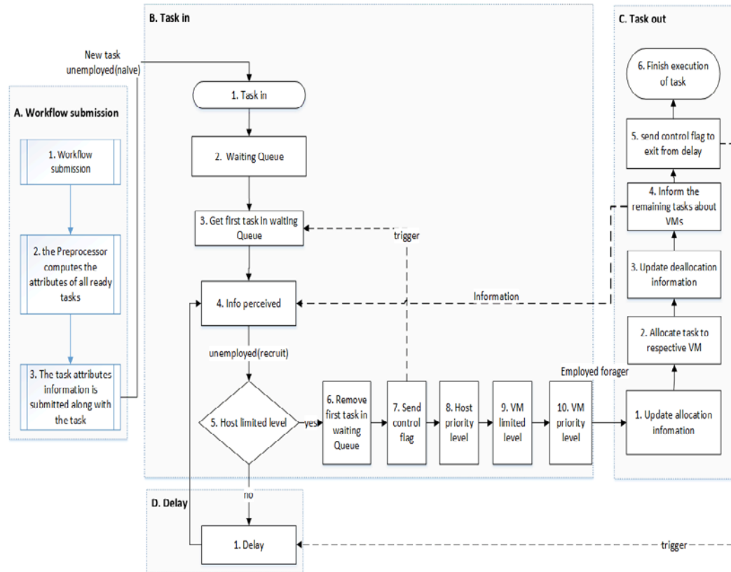
Fig. 2. Flow diagram of the behavioral control structure for LBA_HB.
