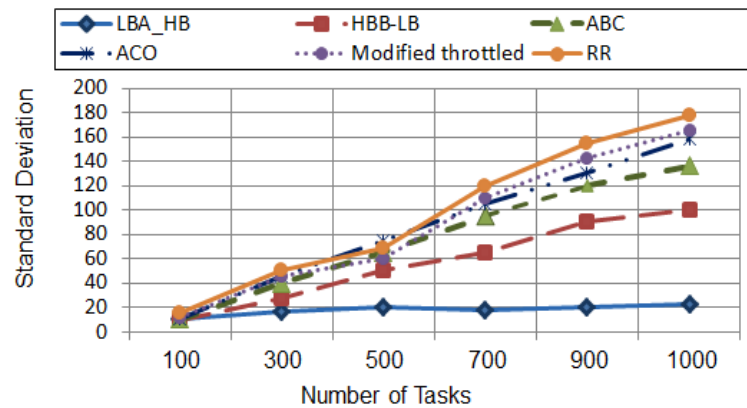
Fig. 11. Standard deviation versus number of tasks.
