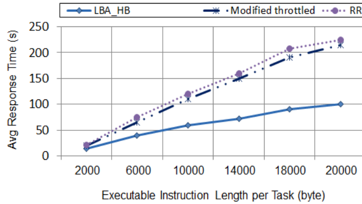
Fig. 7. Average response time with executable instruction length for each task.
