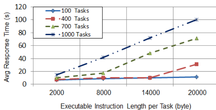
Fig. 5. Average response time of LBA_HB versus executable instruction length at different average number of requests.
