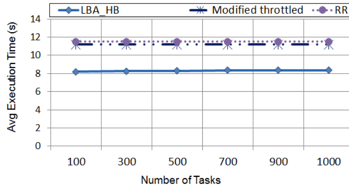
Fig. 8. Average execution time versus number of tasks.
