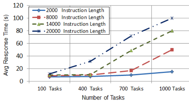
Fig. 4. Average response time of LBA_HB versus number of tasks at different values of instruction length.
