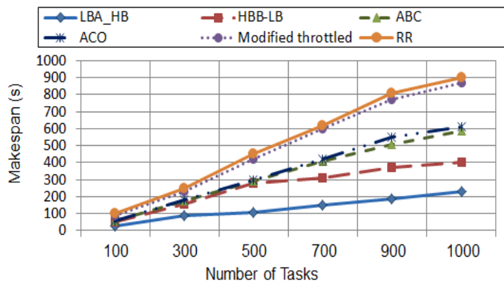
Fig. 10. Average makespan versus number of tasks.
