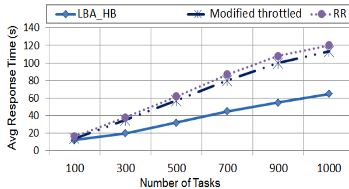
Fig. 6. Average response time versus number of tasks.
