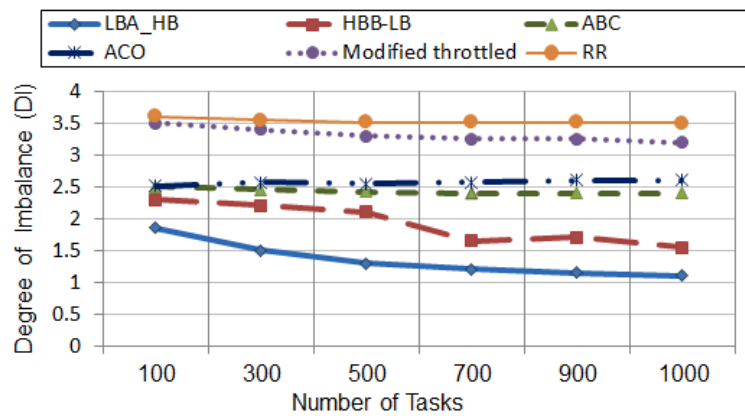
Fig. 9. DI versus number of tasks.
