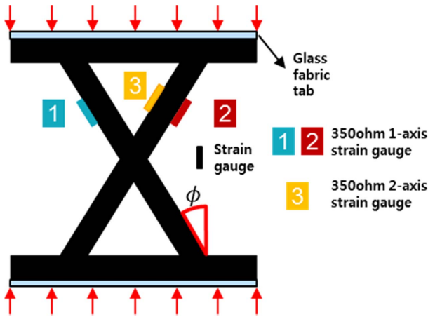
Fig. 4. Single unit cell for compression test
