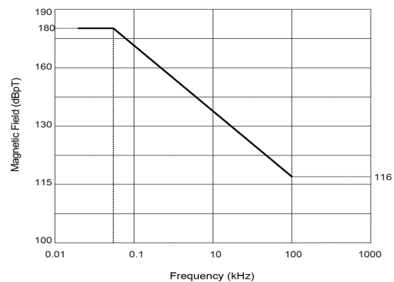
Fig. 2 RS101 test level
