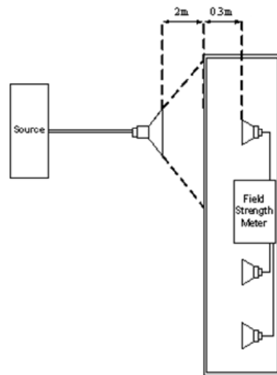
Fig. 3 Method of shield effectiveness measurement (above 1 GHz)
