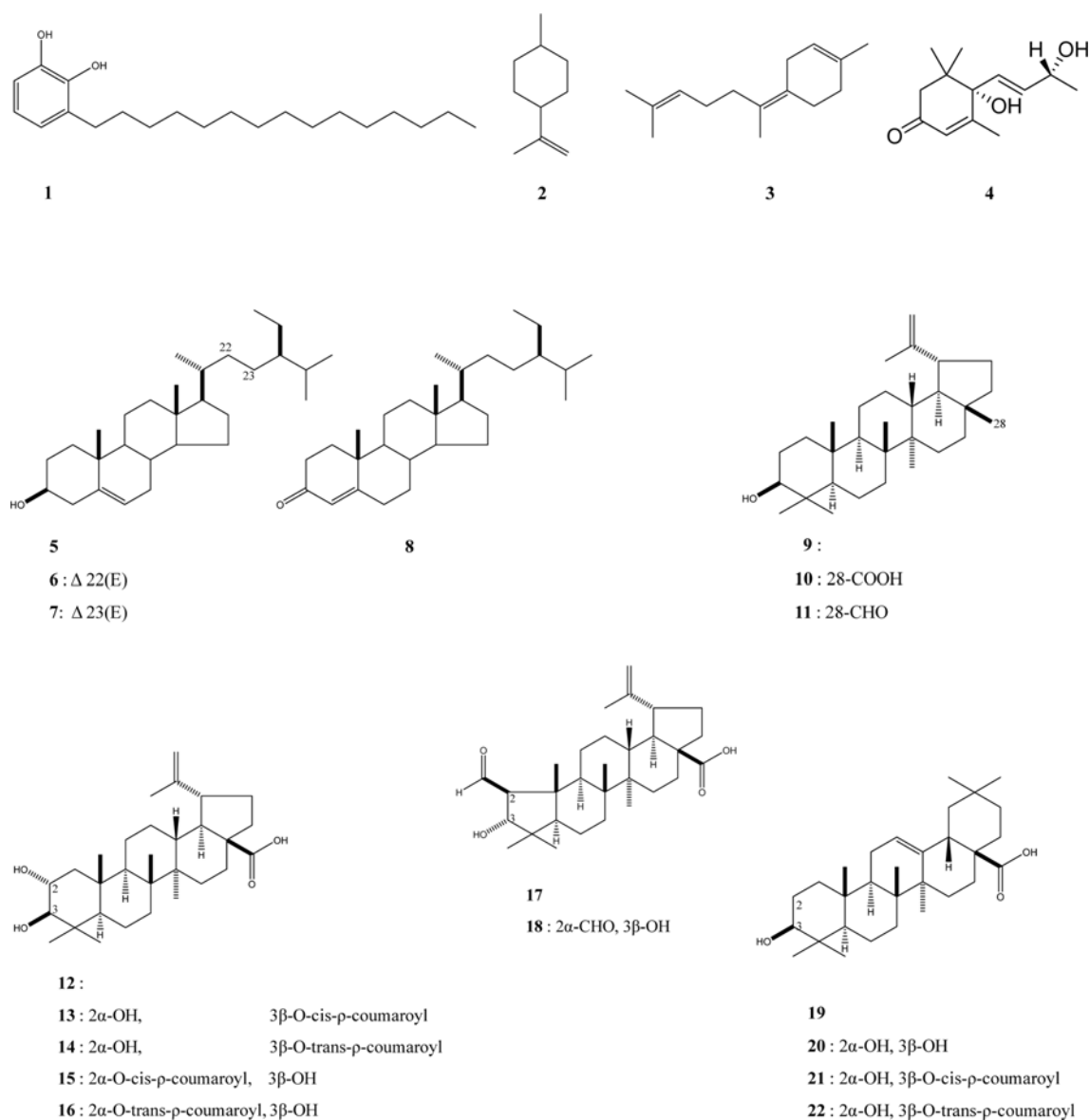
Fig. 1. The structures of compounds (1~22).
