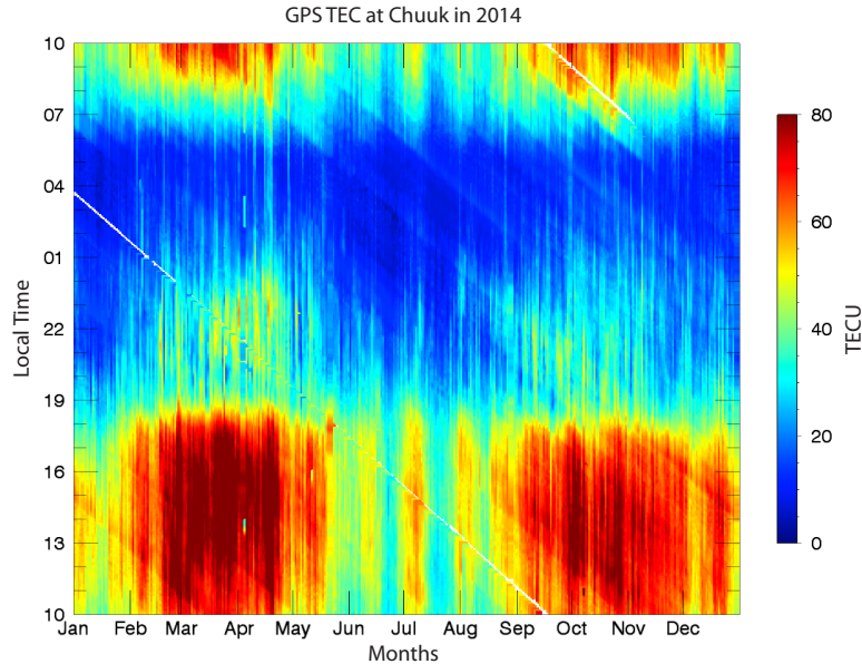
Fig. 3. Local time and seasonal variations of the mean VTEC values measured from the KASI CHUK GPS site during the solar maximum in year 2014.
