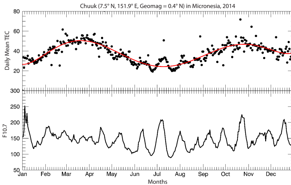
Fig. 2. The daily mean TEC values (solid circle) measured from the KASI CHUK GPS site and its fitting line (red line) and F_{10.7} index under quiet geomagnetic condition ( Kp \leq 3.0 ) in 2014.
