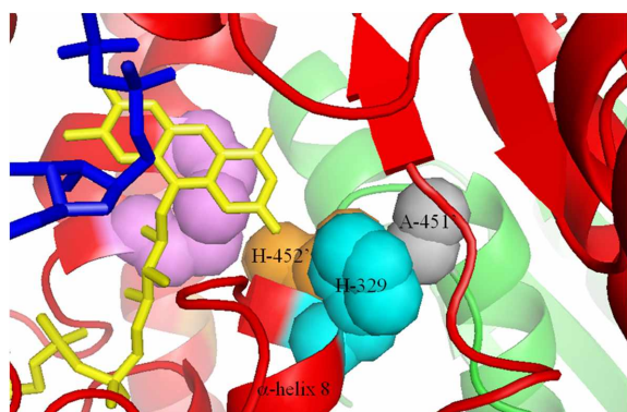
Figure 3. Location of His-329 in human E3. The two subunits of human E3 are shown as cartoons, with each secondary structure portrayed in a single color (red and green, respectively). FAD (yellow) and NAD + (blue) are shown as sticks and the active disulfide center (violet), Ala-451 o (grey), His-452 o (orange) and His-329 (cyan) are shown as spheres. His-329 is located close to FAD and the active disulfide center and can form van der Waals interactions with Ala-451 o and His-452 o from the other subunit. The structure was drawn using the PyMOL program (Delano Scientific LLC). The PDB ID for the human E3 structure is 1ZMC.
