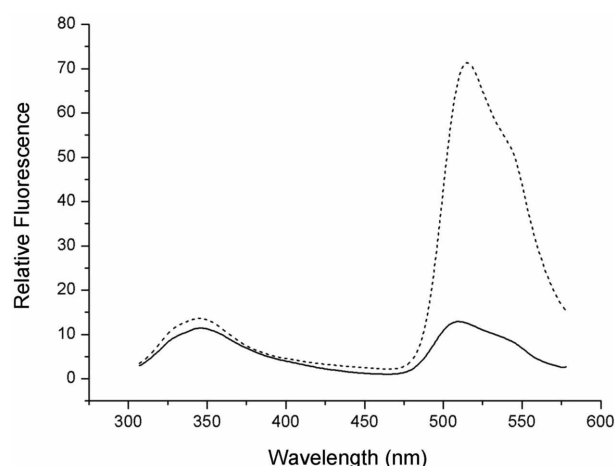
Figure 6. Fluorescence spectra of the wild-type (dotted line) and mutant (solid line) recombinant human E3s. The enzymes were excited at 296 nm and the emissions were observed from 305 nm to 575 nm. The data were transferred to an ASCII file and the spectra were then drawn using the MicroCal Origin program.
