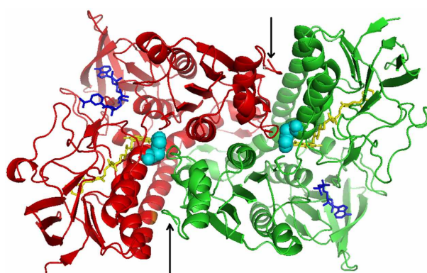
Figure 1. Homodimeric structure of human E3. The two subunits are shown as cartoons, with each secondary structure portrayed in a single color (red and green, respectively). FAD (yellow) and NAD + (blue) are shown as sticks and His-329 (cyan) is shown as spheres. The arrows indicate the dihydrolipoamide binding channels. The structure was drawn using the PyMOL program (DeLano Scientific LLC). The PDB ID for the human E3 structure is 1ZMC.
