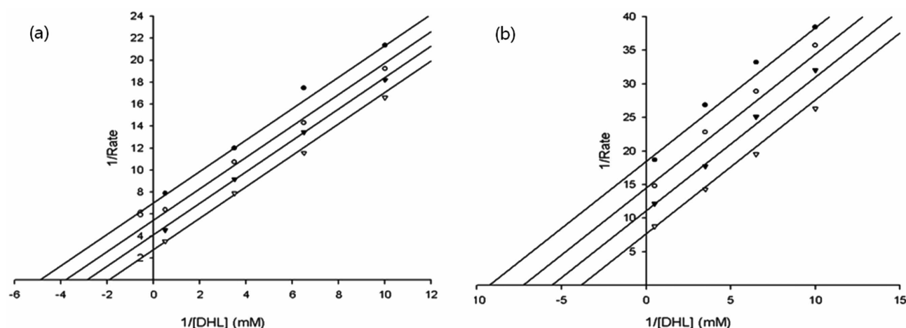
Figure 5. Double reciprocal plots for the wild-type (a) and mutant (b) human E3s. The activities of E3 were determined at 37 °C in a 50 mM potassium phosphate buffer (pH 8.0) containing 1.5 mM EDTA with variable concentrations of the substrates, dihydrolipoamide (DHL) and NAD + . The plots were drawn with the SigmaPlot Enzyme Kinetics Module program. The NAD + concentrations from top to bottom are 0.1, 0.154, 0.286 and 2 mM. The DHL concentrations from right to left are 0.1, 0.154, 0.286 and 2 mM.
