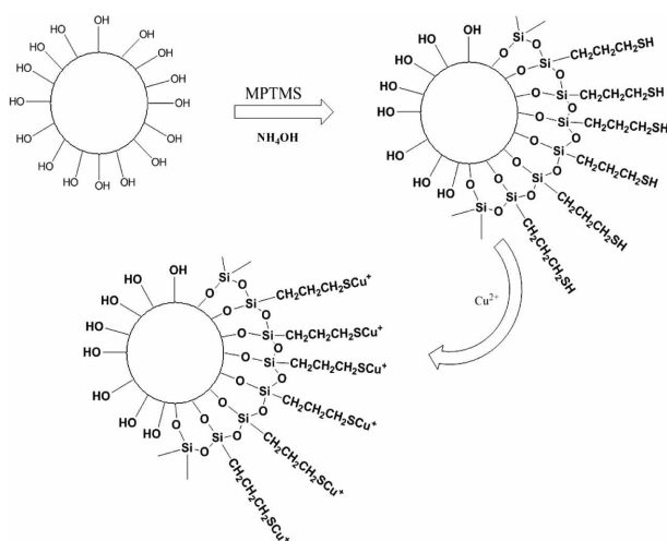
Figure 1. The graphical representation of surface modification of silica spheres and copper uptake process.
