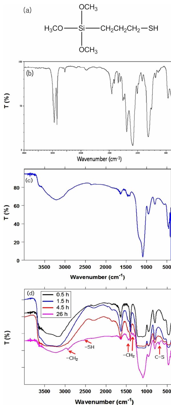
Figure 2. (a) Chemical structure of MPTMS, (b) FTIR spectrum of MPTMS, (c) FTIR spectrum of pure silica spheres, and (d) FTIR spectra of surface modified silica spheres reacted for 0.5, 1.5, 4.5, and 26 h with MPTMS.
