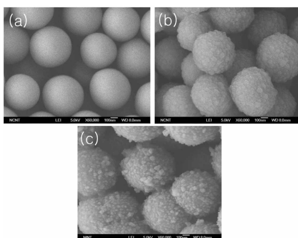
Figure 3. FESEM images of (a) bare silica spheres, (b) surface modified silica spheres with MPTMS, and (c) surface modified silica spheres after treatment with copper solution.
