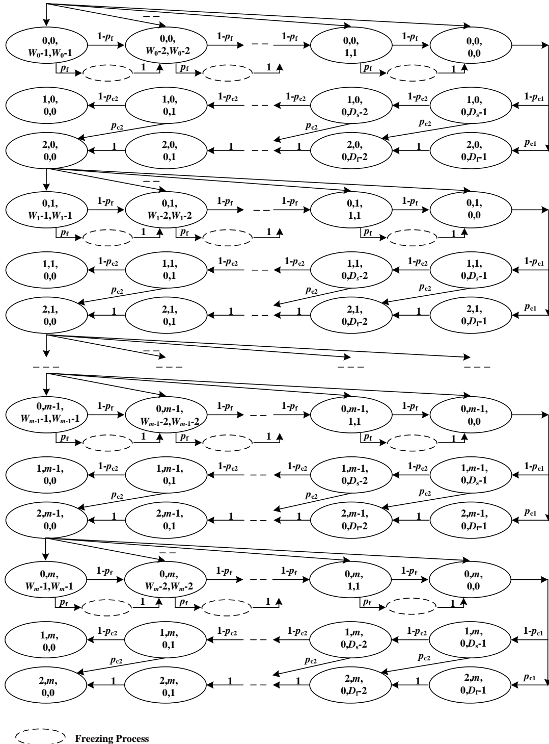
Fig. 3. The total Markov chain model for the tagged node
