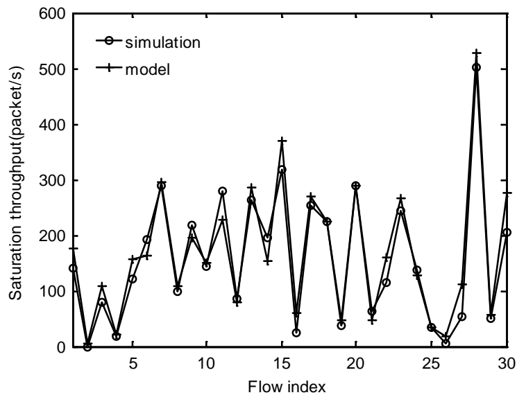
Fig. 14. Saturation throughput of each flow
