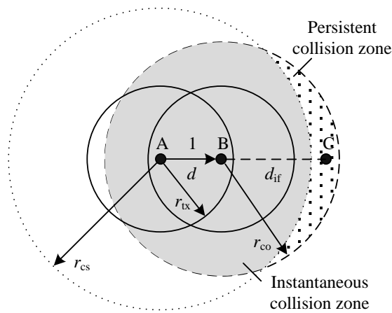
Fig. 1. Collision zones of receiver
