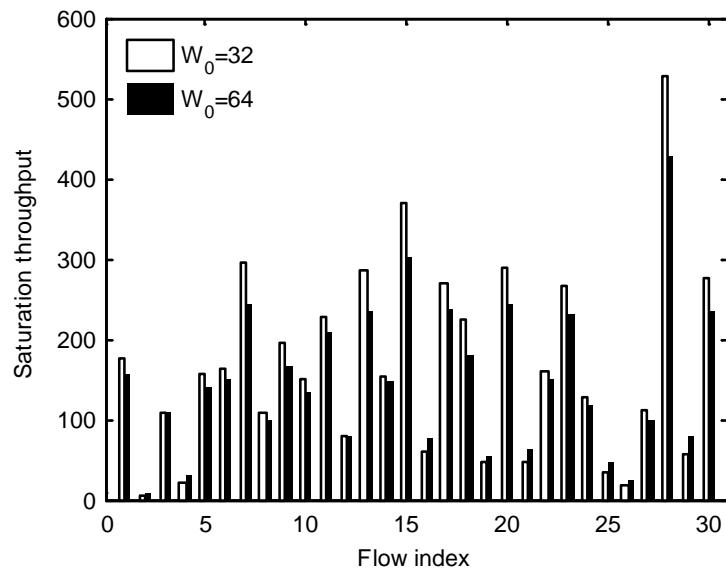
Fig. 15. Throughputs of each flow
