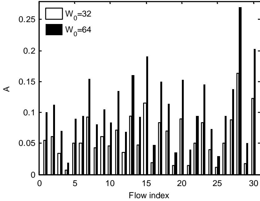
Fig. 9. The probabilities of the nodes being in the backoff progress
