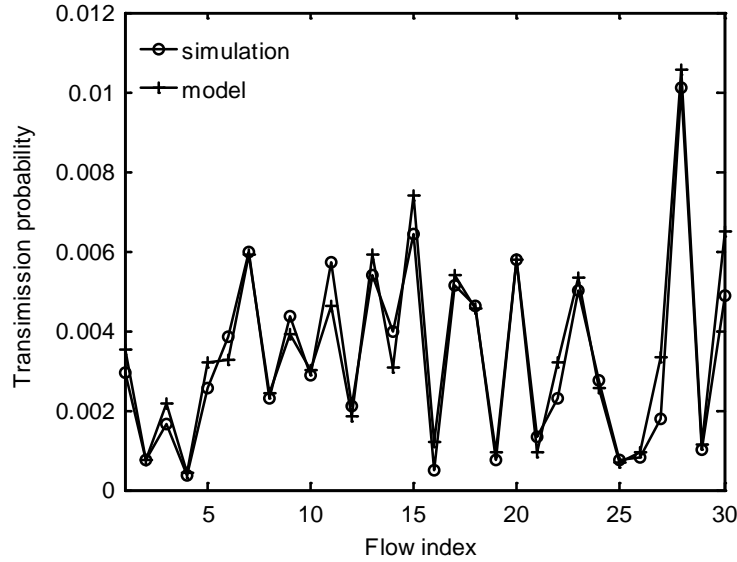
Fig. 6. Transmission probability of each flow
