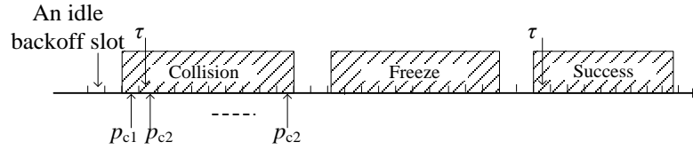
Fig. 2. Redefined performance metrics
