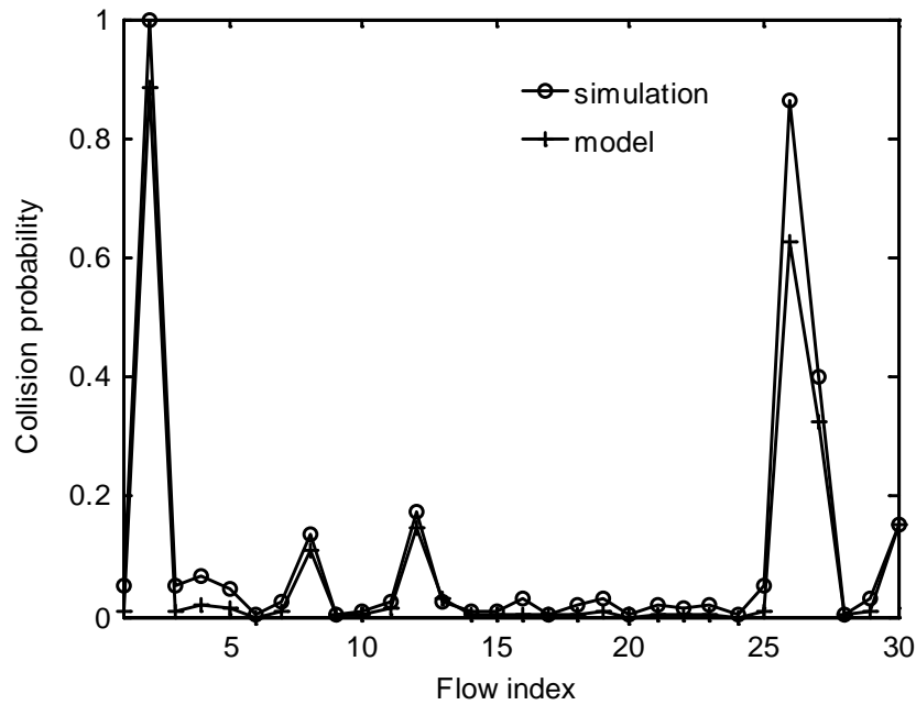
Fig. 12. Collision probability of each flow
