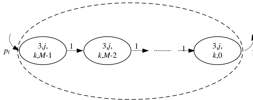
Fig. 4. The freezing process
