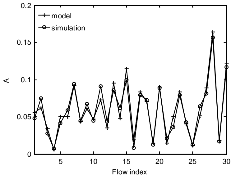
Fig. 8. The probability of the nodes being in the backoff process
