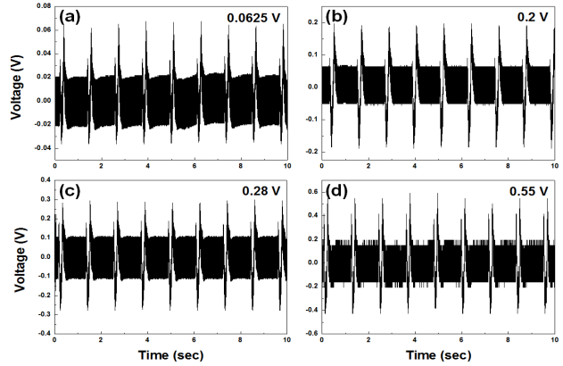
Fig. 4. Generated voltage from the CNT/PVDF composite films with CNT concentration of (a) 0.015, (b) 0.03, (c) 0.05, and (d) 0.075 wt%.
