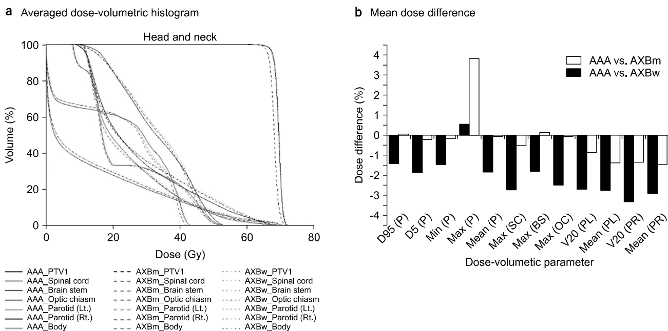
Fig. 1. The averaged dose-volume histograms (DVHs) (a) and the mean values of the relative dose differences (b) for PTV and normal tissue in the case of head and neck. Solid lines, dotted lines, and dashed lines are for DVHs calculated by AAA, AXB w and AXB m , respectively. The D n% (structure) means dose received n% volume of certain structure. V n Gy (structure) means the percent volume of certain structure irradiated by at least n Gy. The minimum dose, maximum dose, and mean dose were abbreviated to min, max, and mean, respectively. The PTV, spinal cord, brain stem, optical chiasm, left parotid gland and right parotid gland were abbreviated to P, SC, BS, OC, PL and PR, respectively.
