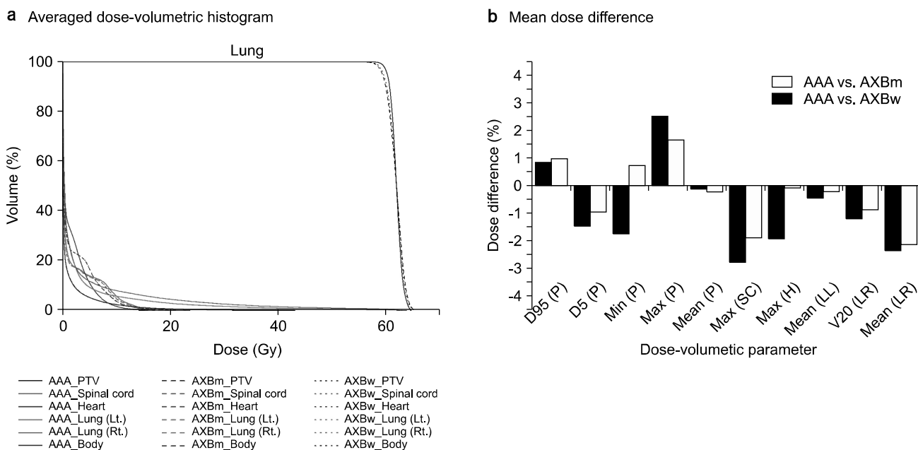
Fig. 4. The averaged dose-volume histograms (DVHs) (a) and the mean values of the relative dose differences (b) for PTV and normal tissue in the case of lung. Solid lines, dotted lines, and dashed lines are for DVHs calculated by AAA, AXB w and AXB m , respectively. The D n% (structure) means dose received n% volume of certain structure. V n Gy (structure) means the percent volume of certain structure irradiated by at least n Gy. The minimum dose, maximum dose, and mean dose were abbreviated to min, max, and mean, respectively. The PTV, spinal cord, heart, left lung, and right lung were abbreviated to P, SC, H, LL, and LR, respectively.
