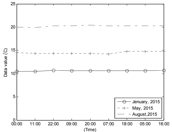
Fig. 21. Underwater Temperature
