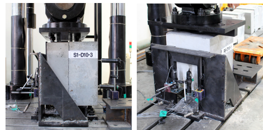
Fig. 5. Views of Shear Test
