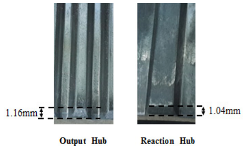
Fig. 16. Measurement of non-forming area
