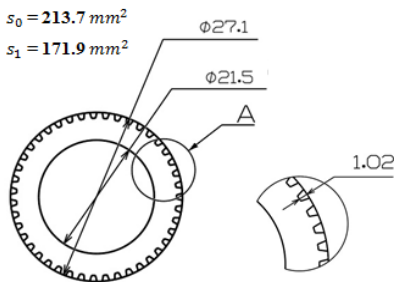
Fig. 15. Reduction area of output hub and reaction hub
