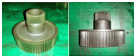
Fig. 2. Output hub of automatic transmission
