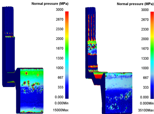
Fig. 14. Normal pressure of output hub & reaction hub
