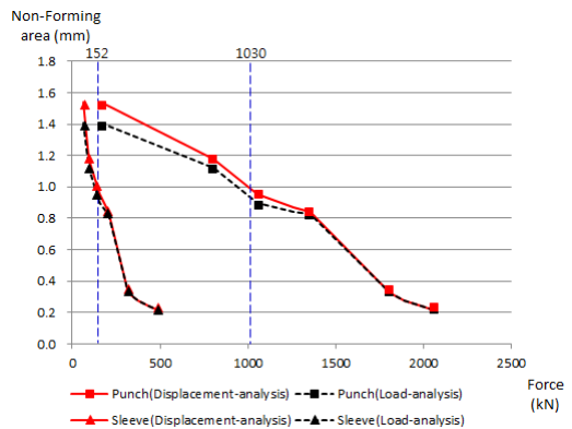
Fig. 13. Non-forming area vs. reaction force of reaction hub
