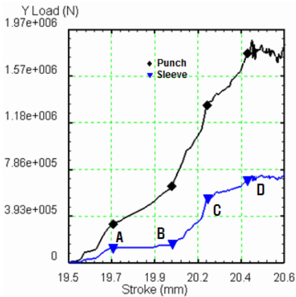
Fig. 6. Load-stroke curve of output hub
