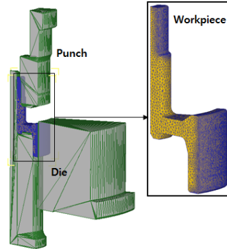
Fig. 5. Finite element model
