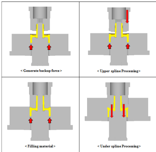
Fig. 4. Process of back-pressure cold forging
