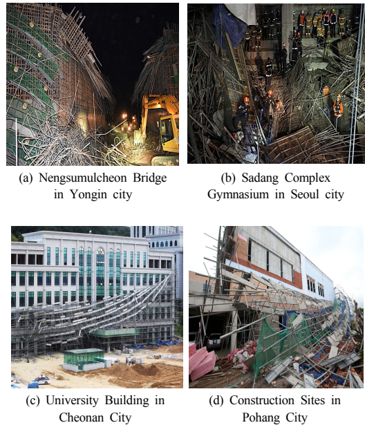
Fig. 1. Failures induced by inappropriate use of temporary equipments and materials
