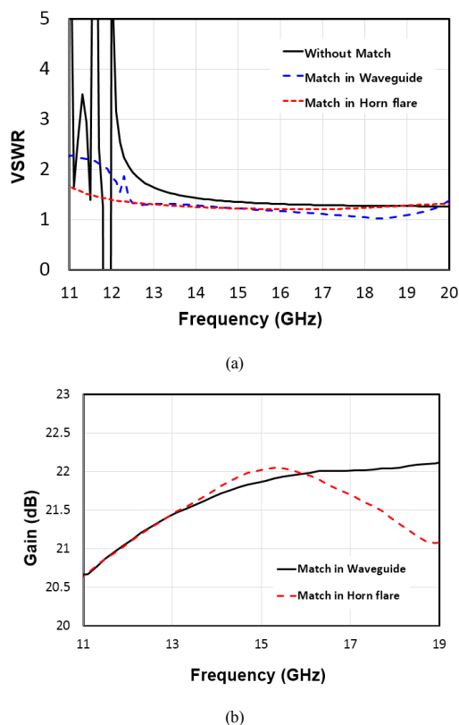
Fig. 5. VSWR and gain characteristics (a) VSWR (b)Gain
