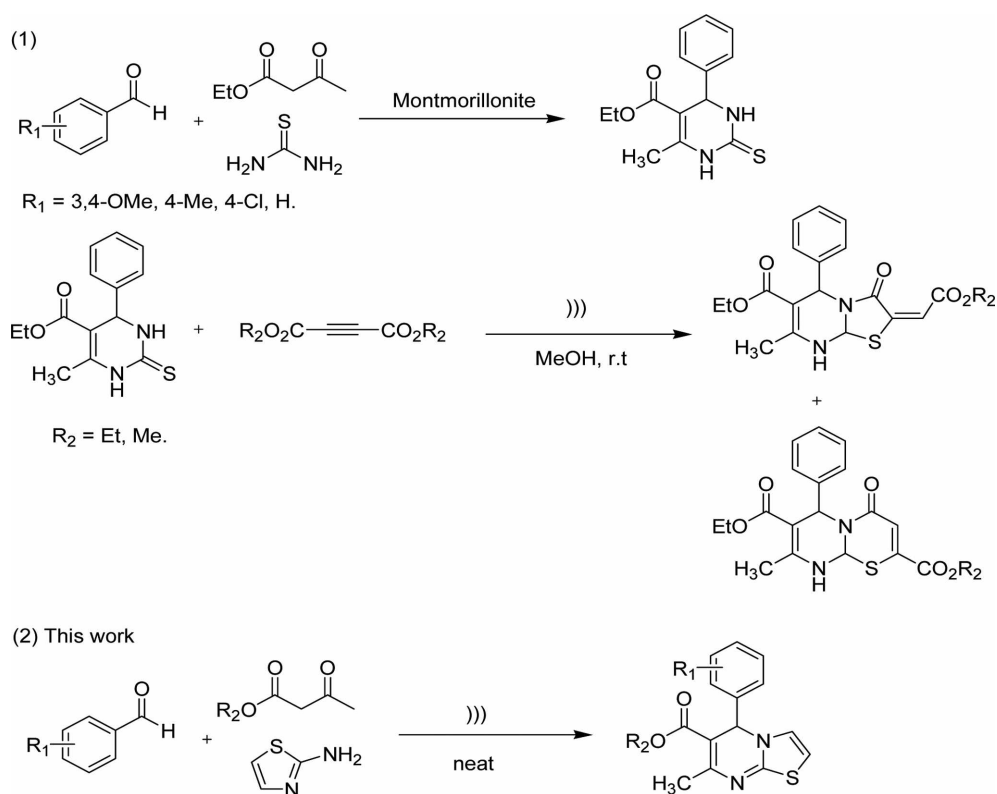
Scheme 1. Synthetic route towards the preparation of thiazolo[3,2-a]pyrimidine-6-carboxylate derivatives.
