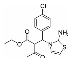
Figure 1. The minor product 11 produced in this procedure.
