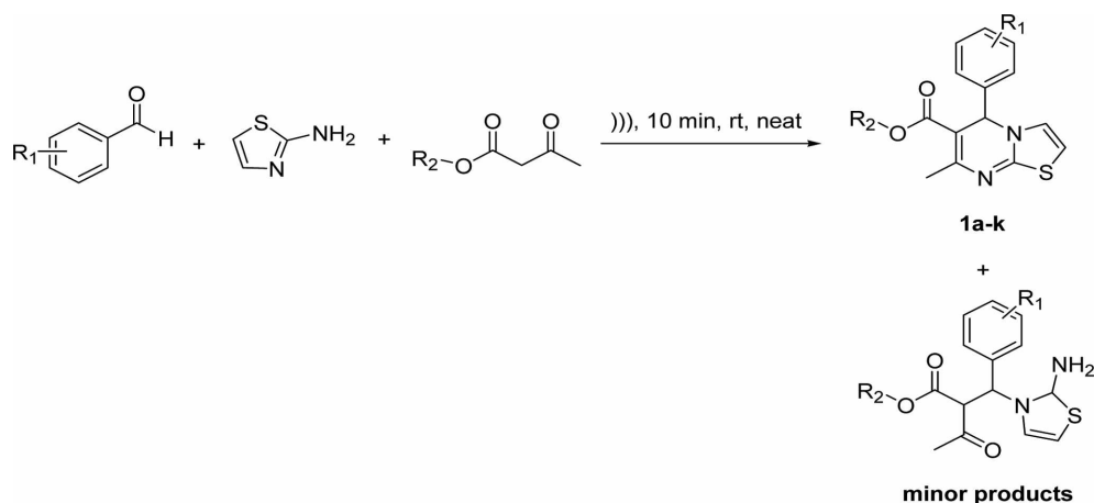
Scheme 2. Synthetic route towards the designated compounds ( 1a-k ).
