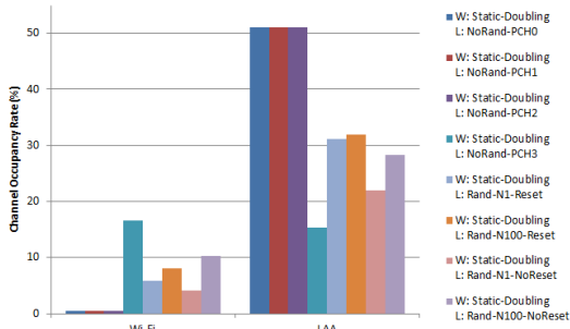
(a) Without a channel bonding rule
