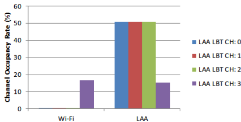
(a) Without a channel bonding rule
