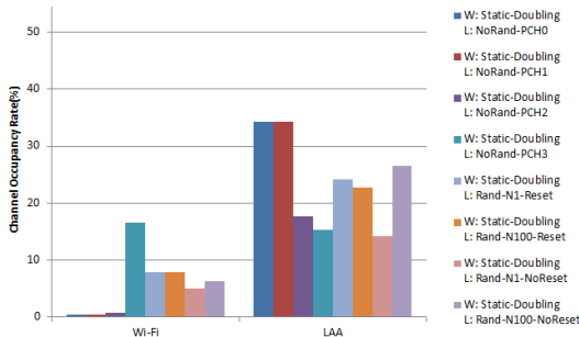
(b) With a channel bonding rule
